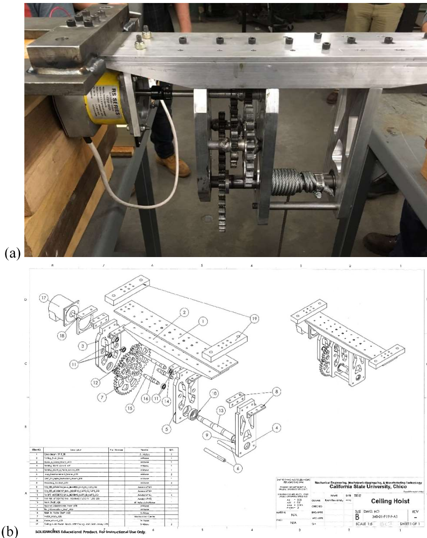
FIGURE 5 ELECTRIC CEILING HOIST FROM GROUP 2; (A) TESTING, (B) ASSEMBLY
