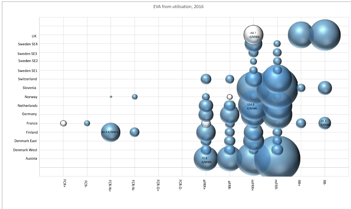
FIGURE 2 EVA 2016 FROM UTILISATION FOR TSO GRID SERVICES
